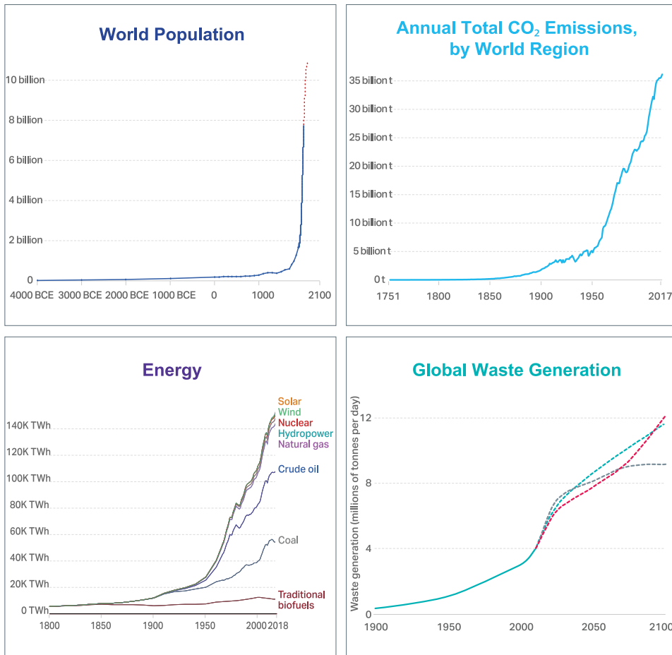
Figure 1: Exponential Growth 2,3
